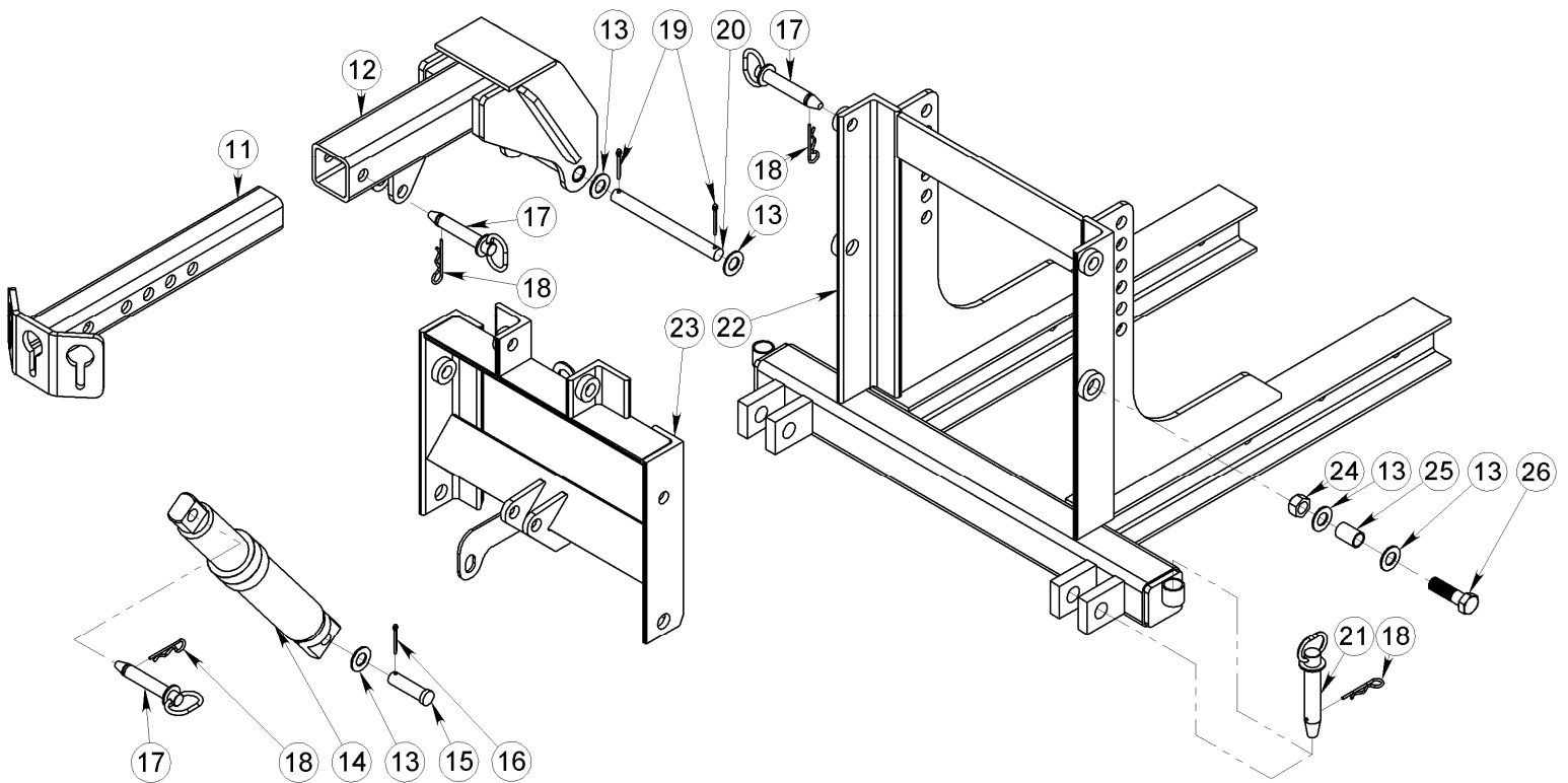
FIGURE 4 – Tilt Hitch w/ Fold-Down Arm (Pin-On Hitch Lift Frame Model Shown)
