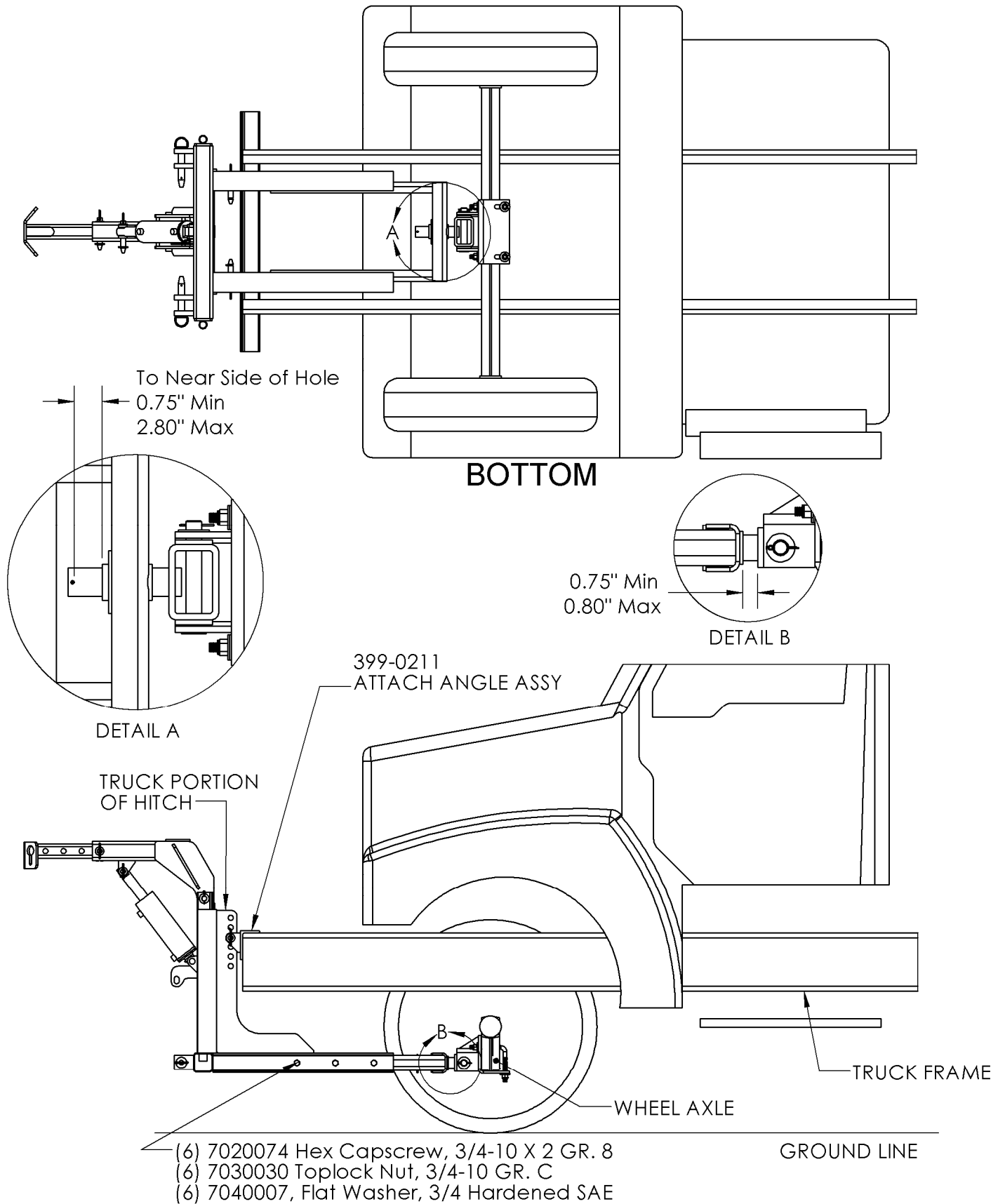
LEFT FIGURE 9 – Typical Hitch Mounting, Axle Saddle Assembly View 1 of 2
