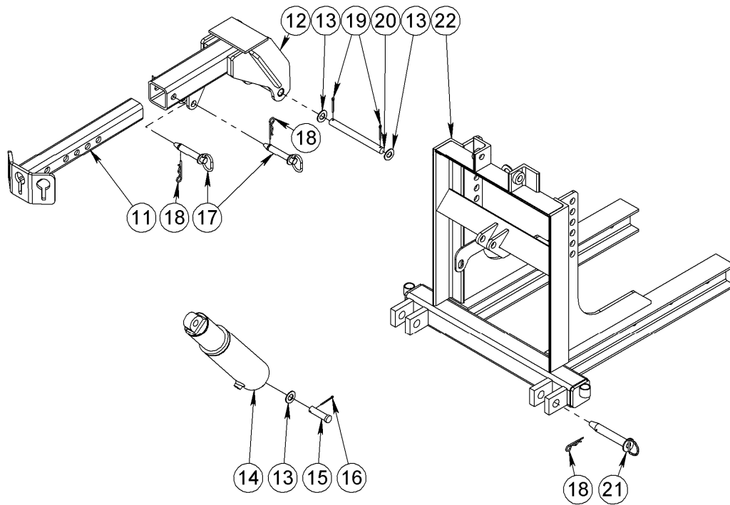
FIGURE 3 – Non-Tilt Hitch w/ Fold-Down Arm (Pin-On Hitch Lift Frame Model Shown)
