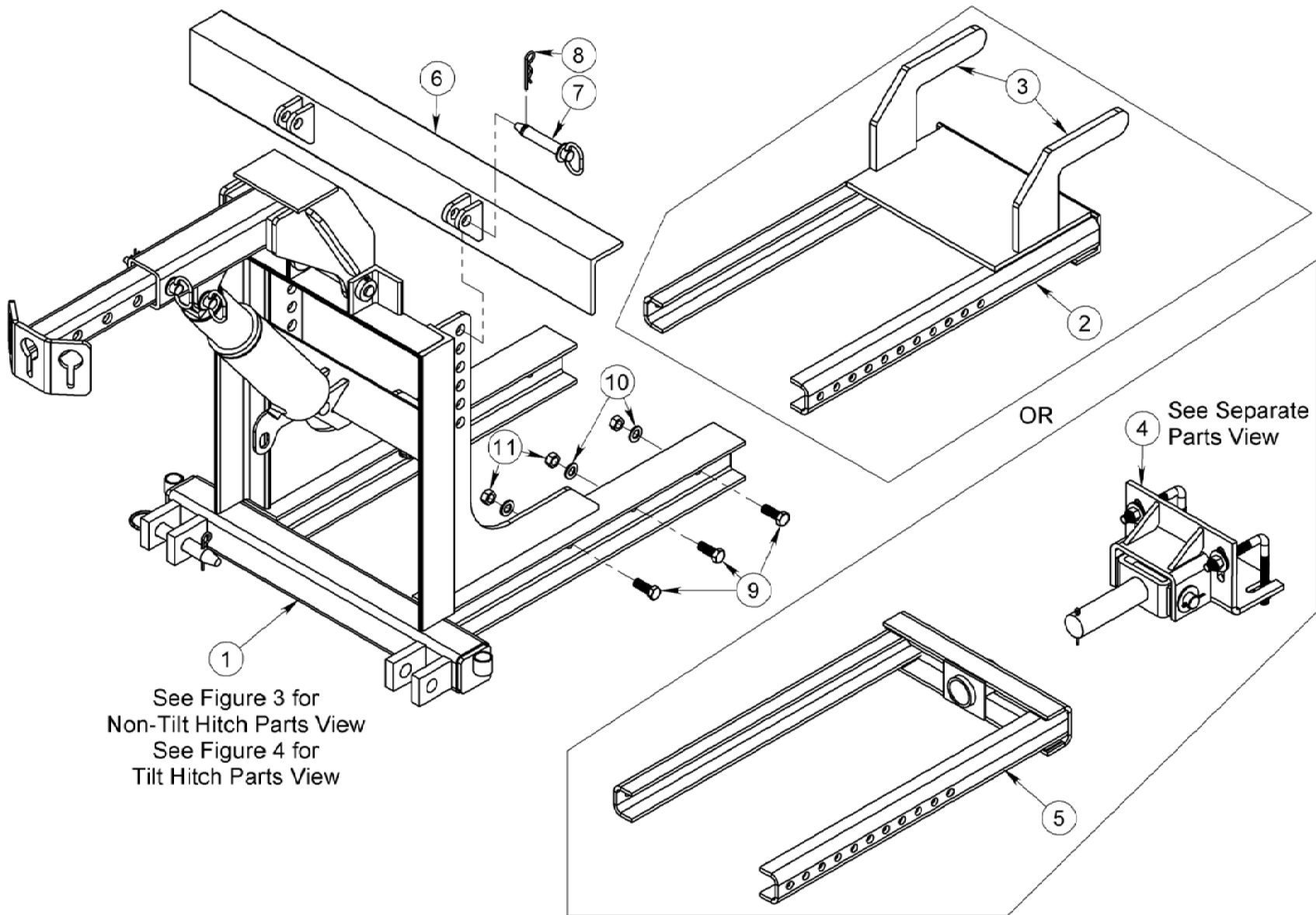
FIGURE 2 – Bumper to Axle, Low Profile Lift Frame w/ Fold-Down Arm, Axle Hooks and Saddle Options Shown On Non-Tilt Universal Pin-On Assembly Model
