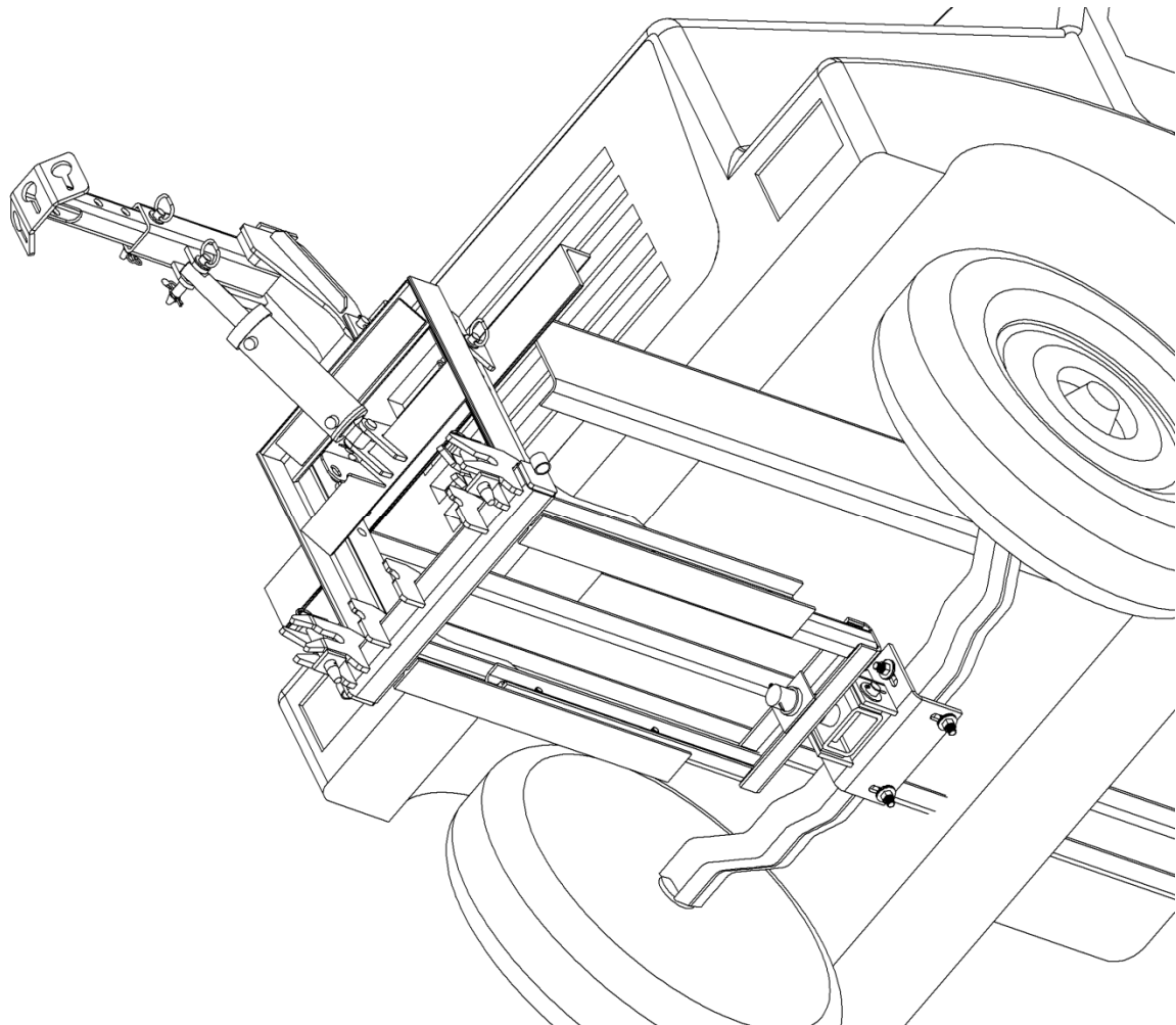
FIGURE 10 – Typical Hitch Mounting, Axle Saddle Assembly, View 2 of 2
