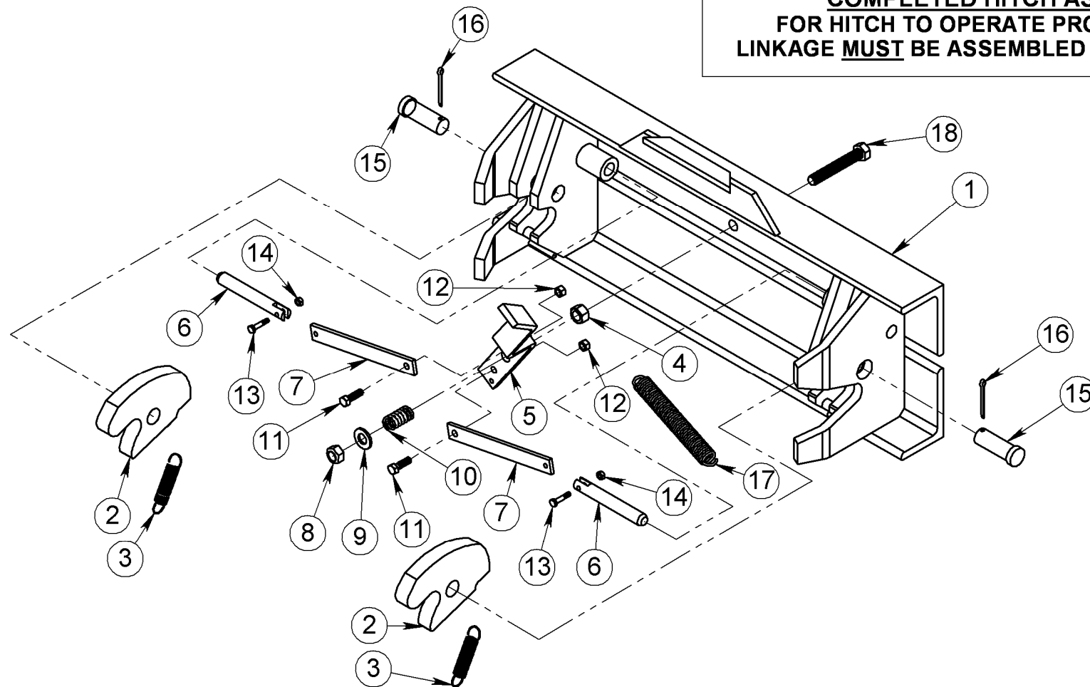
FIGURE 7 – Quick-Link Sub-Assembly
