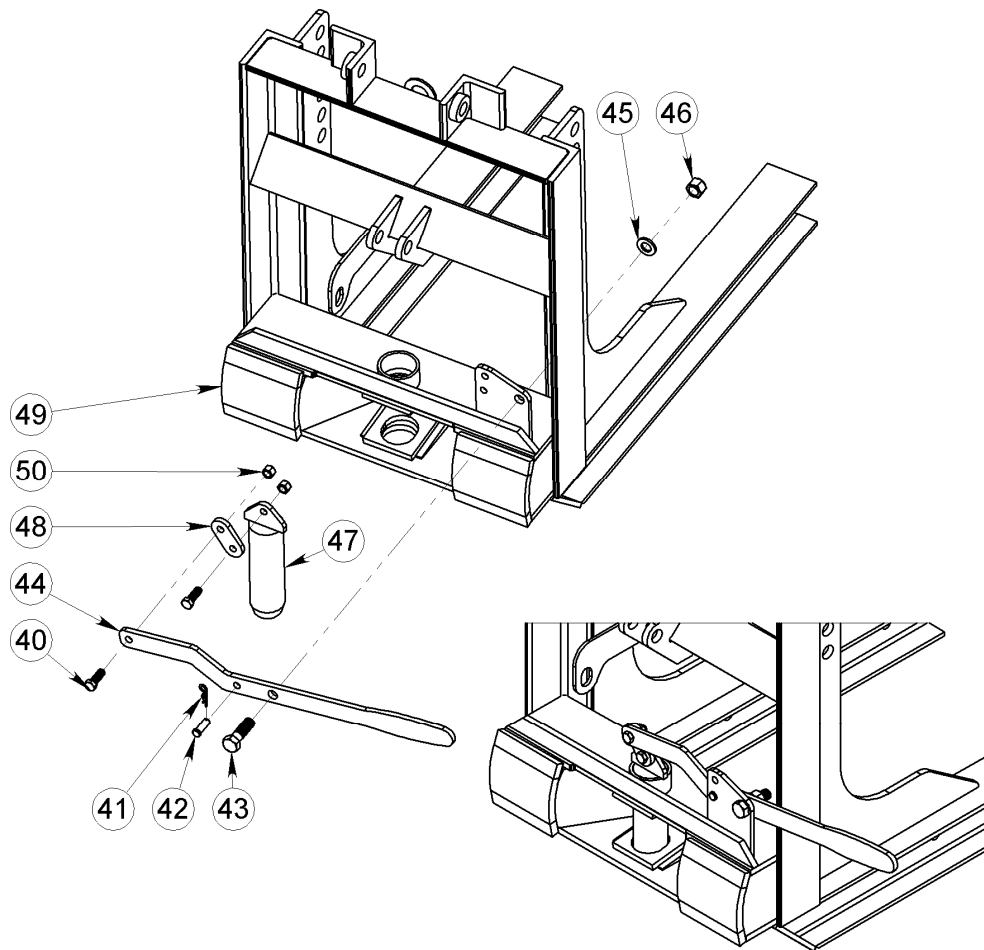
FIGURE 6 – QCP Sub-Assembly
