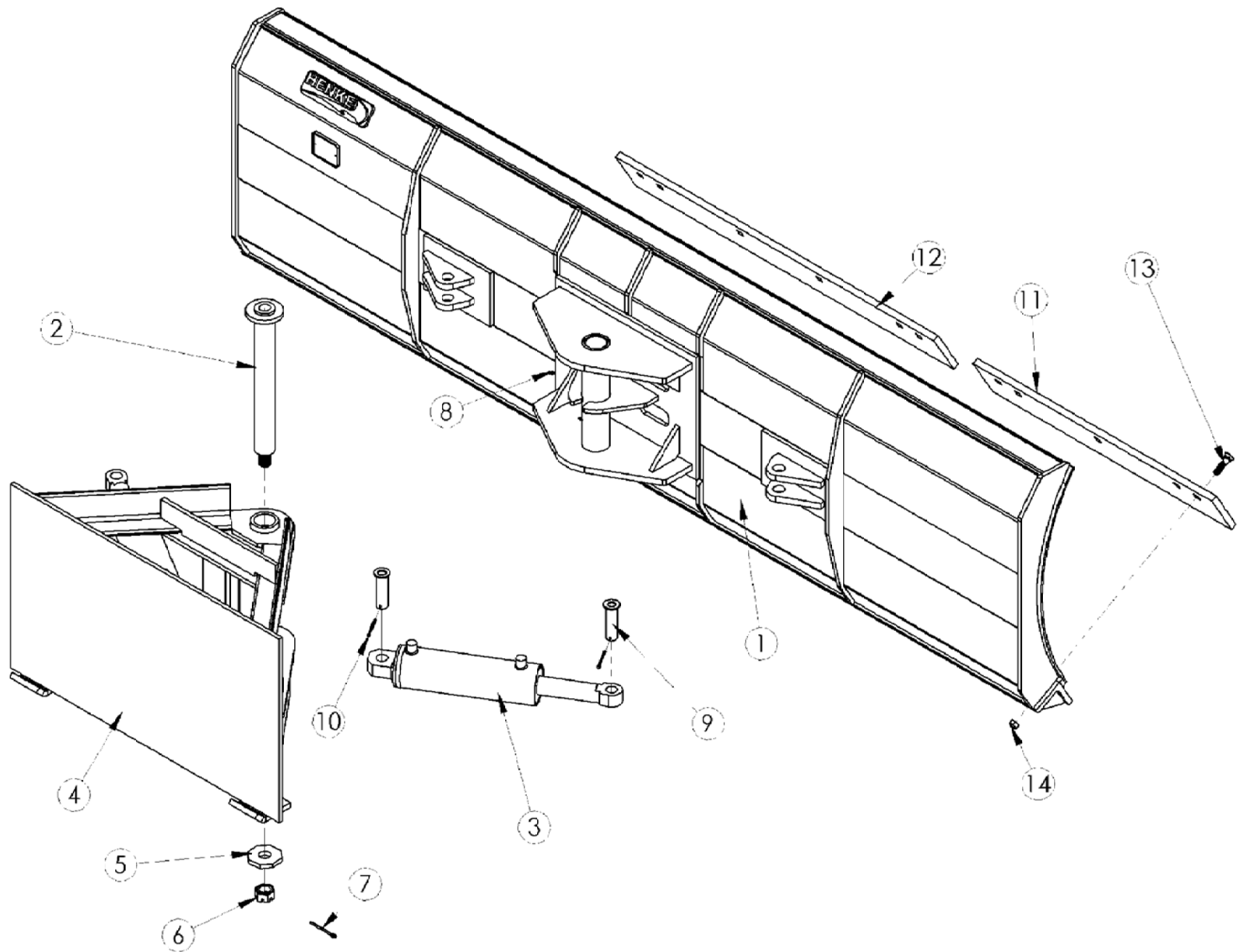
Figure 1 – Exploded View: Henke Helper HH30R
